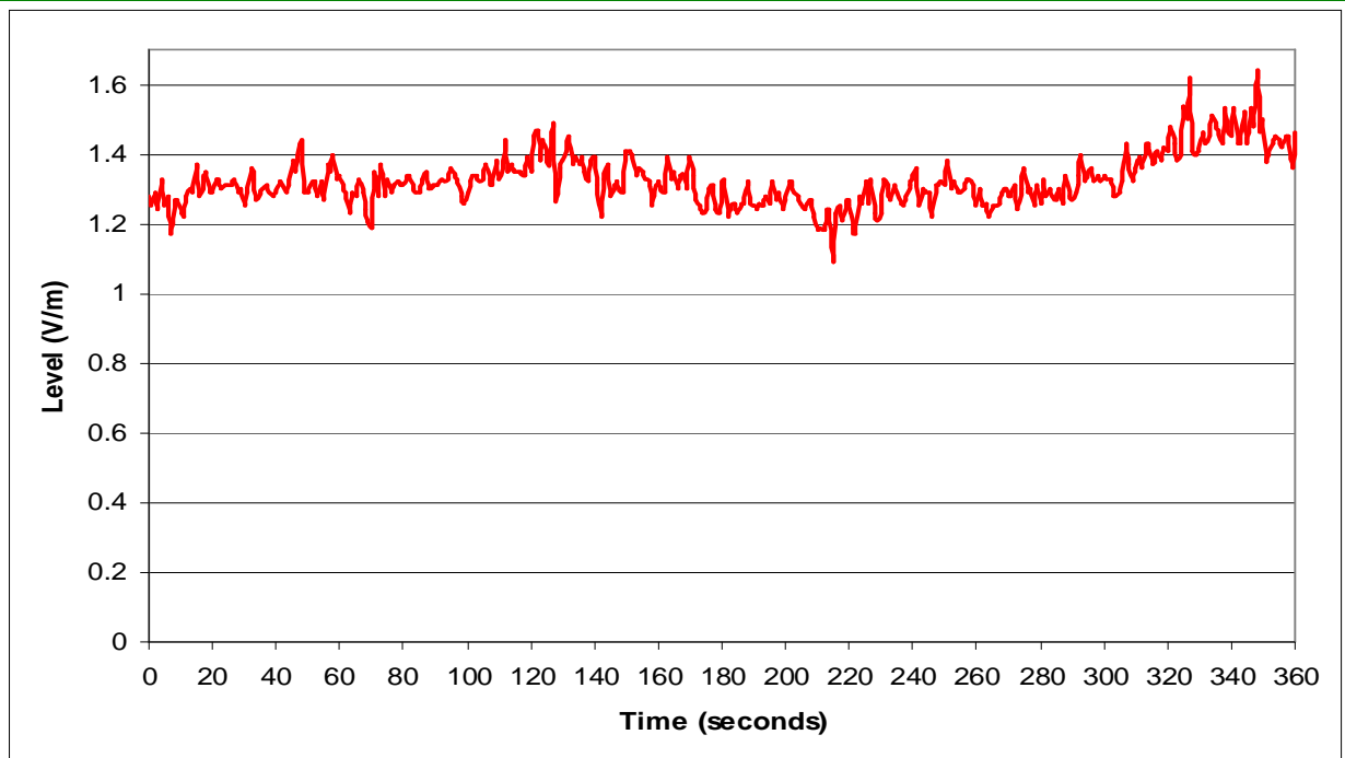
Electric field strengths recorded over 6 min period using 3 GHz probe at point of max NIR:
